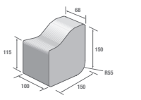
External Radius Block Splay MK/E
