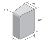
BN Upright Internal/External Radial Block LK/B
