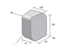
Internal/External Radius Block Bull Nose MK/F
