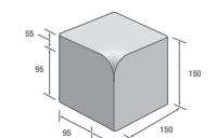
Internal Angle Bull Nose MK/B
