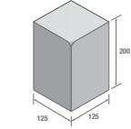
BN Upright Internal Angle LK/F
