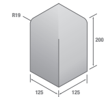
BN Upright External Angle LK/G
