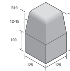
HB Upright External Angle LK/E
